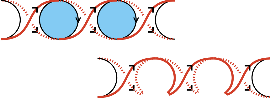
Figure 7: Heirarchies: the inductive step
