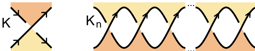
Figure 6: K to K_n
