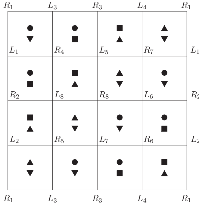
FIGURE 7. Singularization of E -squares
