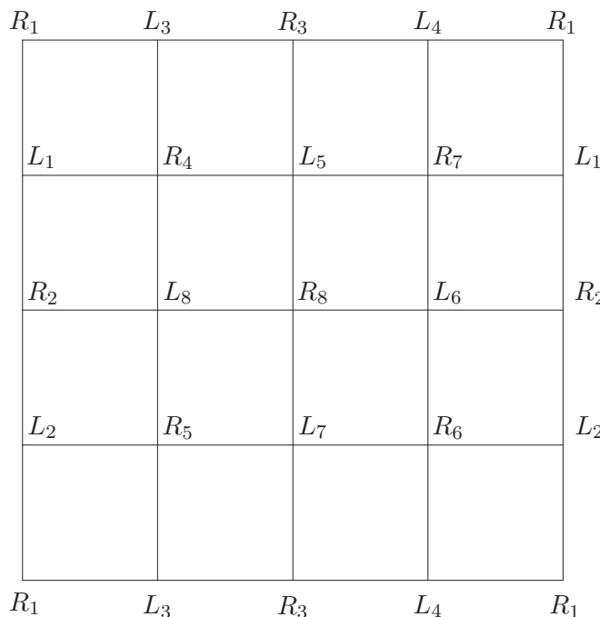
FIGURE 3. The graph \Gamma
