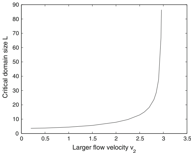
Fig. 6 The relation between the critical domain size and v_2 for the alternating kernel model with v_1 = 0.1, R_1 = 1.2, R_2 = 1.5, D_1 = D_2 = 1 , and \beta_1 = \beta_2 = 1 . As v_2 \rightarrow 3 , the critical domain size approaches infinity
