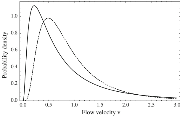
Fig. 9 Probability density functions for a log-normal distribution with fixed mean \bar{v} = 0.95 and variance v = 1.5 (solid) and 0.5 (dashed). Note that the occasional higher flow values for the higher variance case are balanced by more frequent lower flow rates in order to keep the mean fixed
