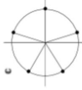
Fifth Roots of Unity
